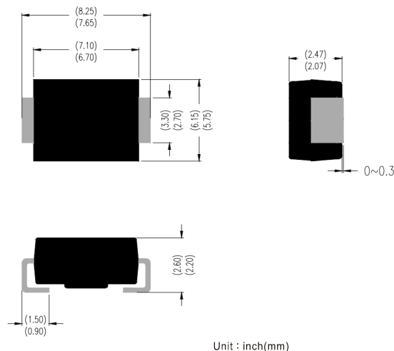
SMC/ DO-214AB
